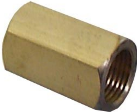
1/4-27 Female by 7/16-24 Female Brass Adapter 24C0-21F-31F
